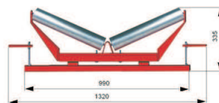
2R1C/1000
