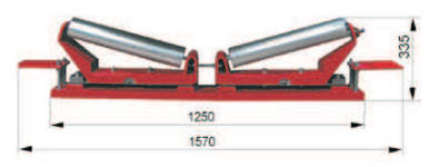
2R2C/1200
